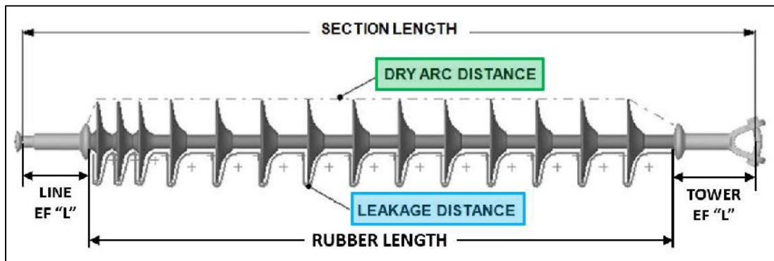
Fig. 23: Polymer Design Dimensions
