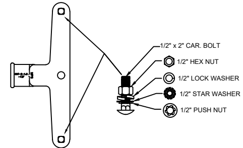
END FITTING VIEW -DDW, -DDWC SUFFIX ->CAT-0-1.5-12FWH (OPTIONAL) W/ HARDWARE
