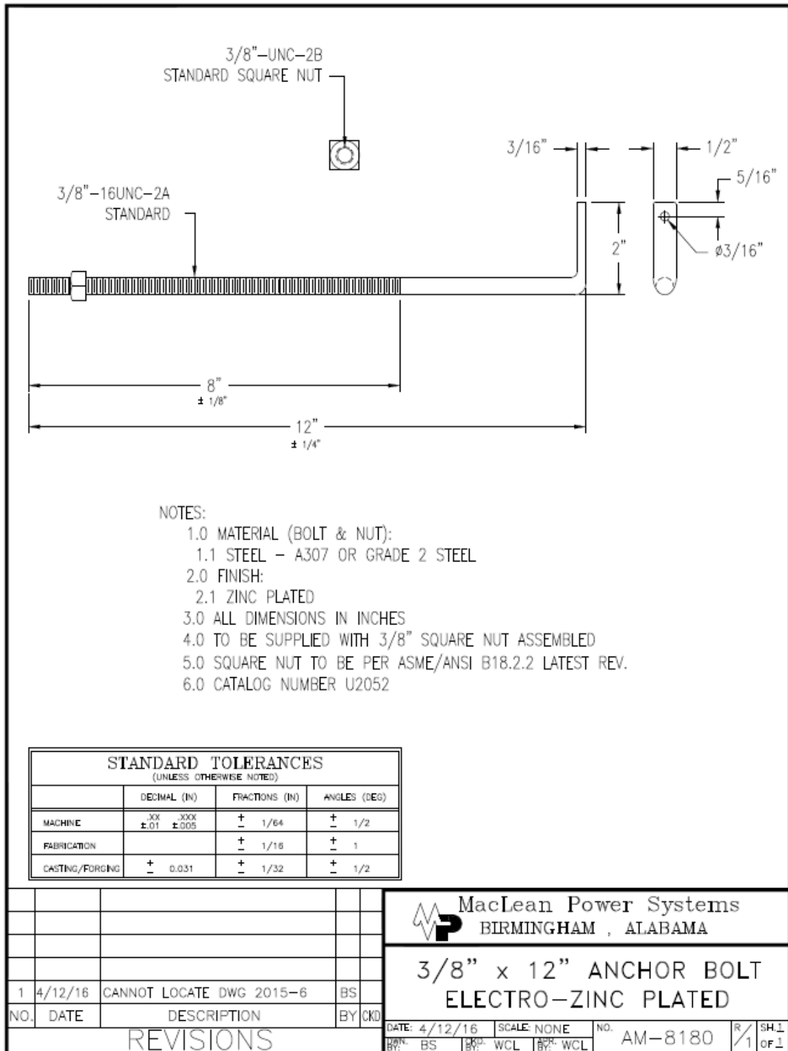
Figure 1 – Anchor Bolt Series Drawing
