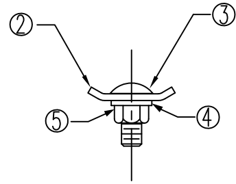
— GROUNDING DETAIL —
