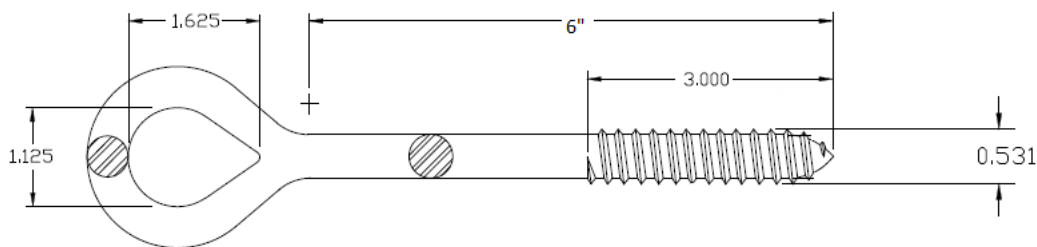
Figure 1 - J8930 Oval Eye Screw
