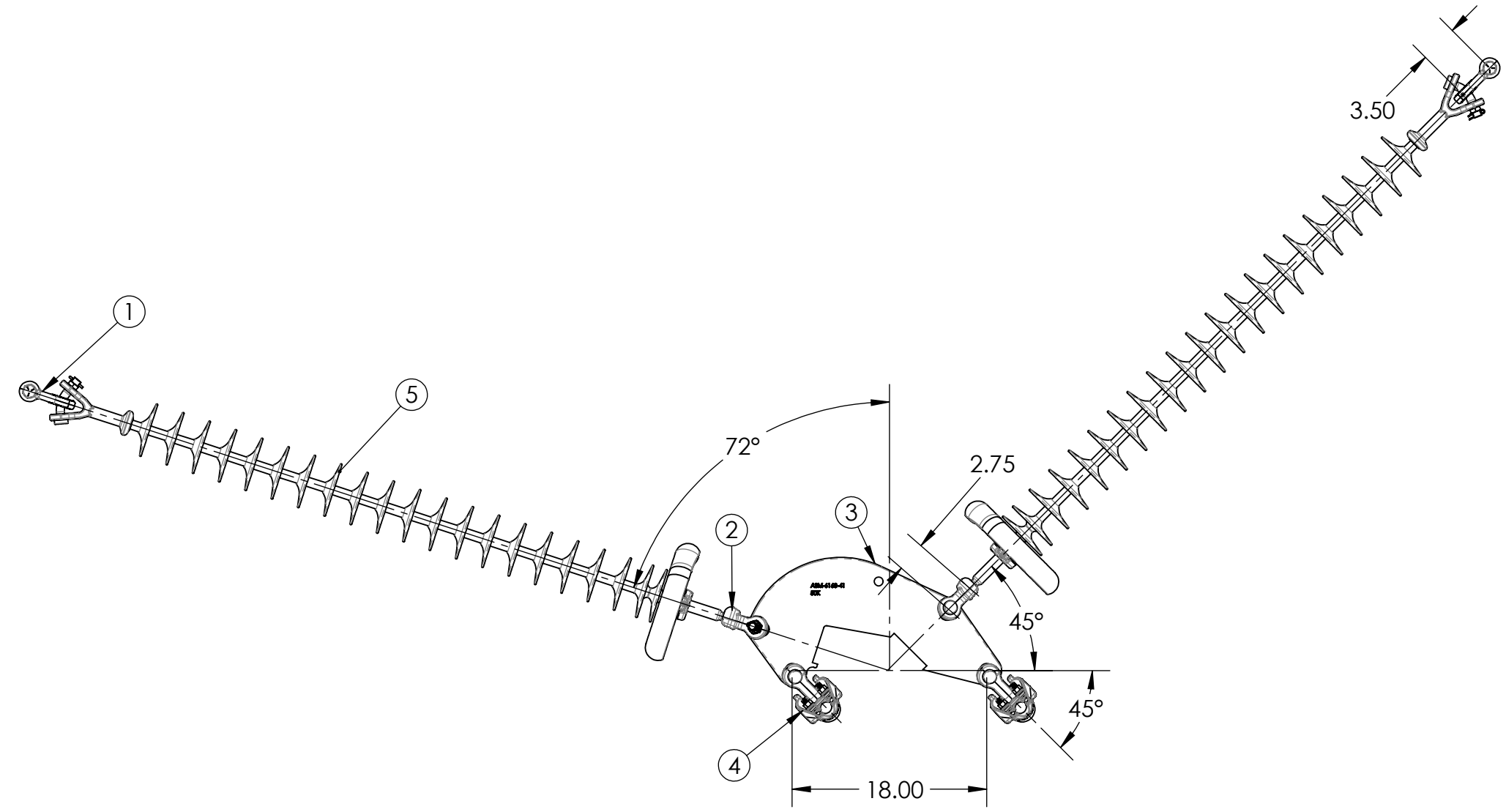
ASSEMBLY CAT. NO. X3RV2YB30A2
